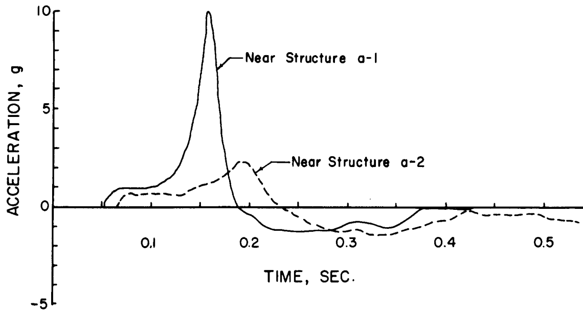
Fig. 8—Medium acceleration vs. time.
